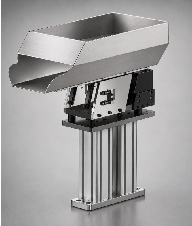
VIBRATORY HOPPERS
